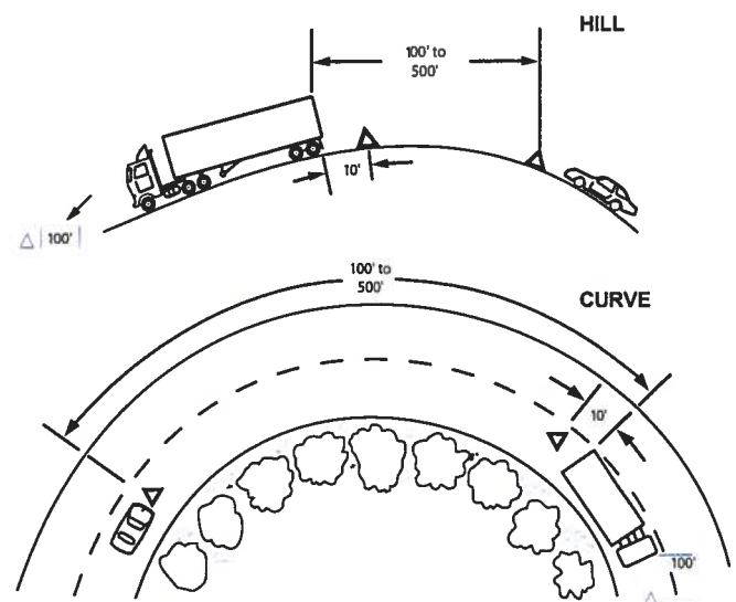
Figure 2-6: Warning Device Placement: Obstructed View
