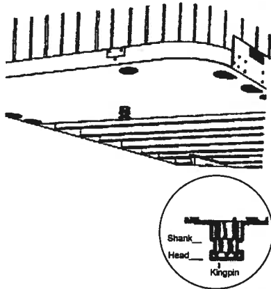
Figure 6-7: Trailer Kingpin
