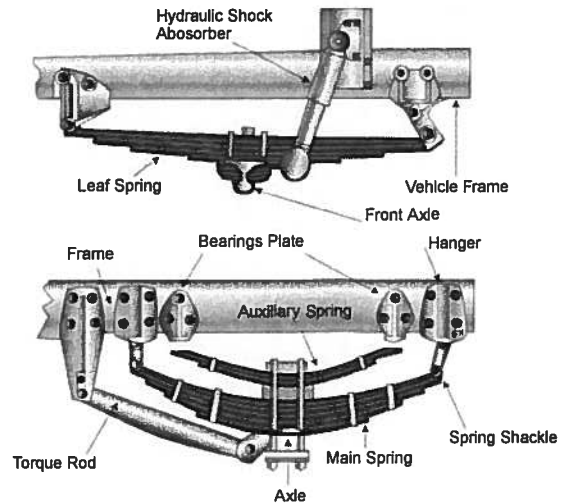
Figure 2-3: Safety Defect: Broken Leaf in Leaf Spring
