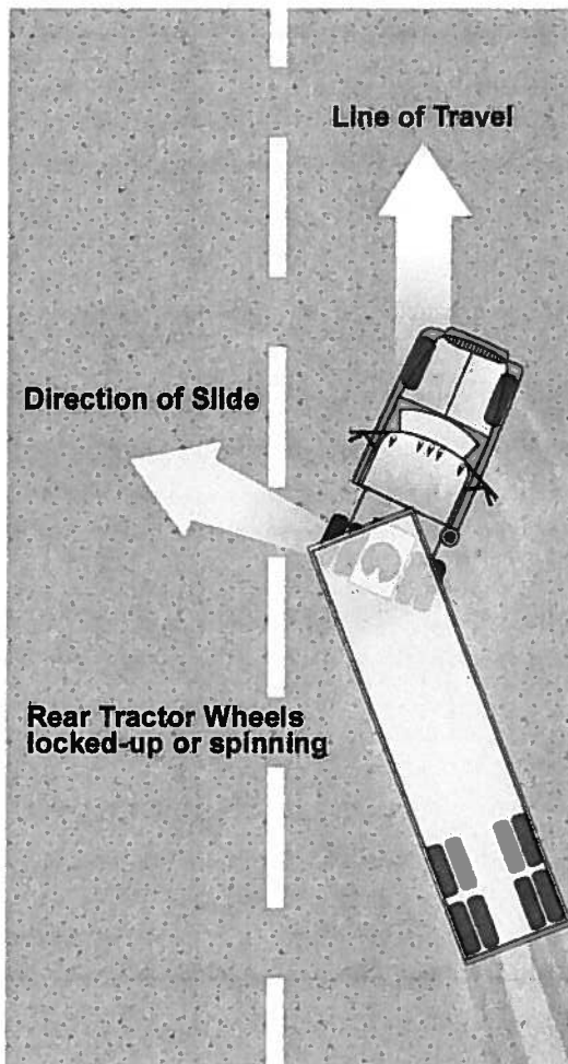
Figure 6-2: Tractor Jackknife
