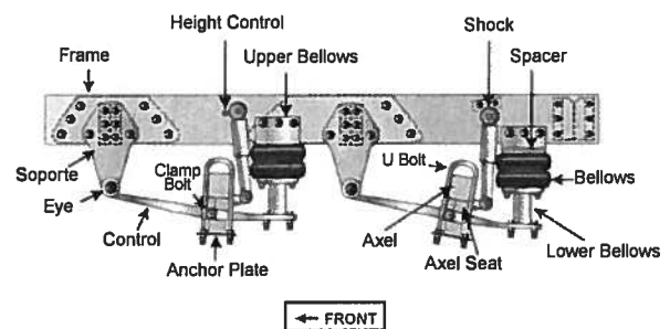
Figure 2-4: Air Suspension Parts
