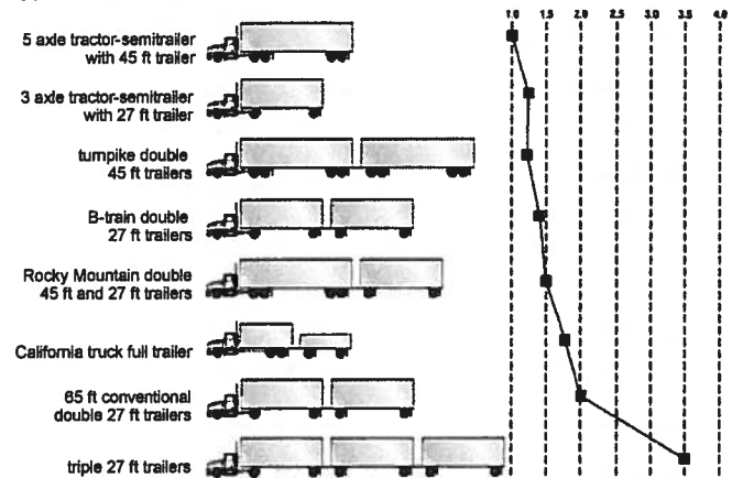
Figure 6-1: Influence of Combination Type on Rearward Amplification
